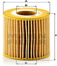
Oil Filter HU 821 x EM-10039
